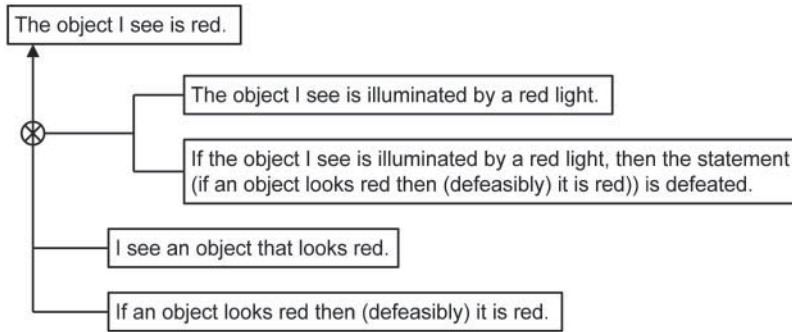
Figure 1. Pollock's red light example modelled in DefLog.
