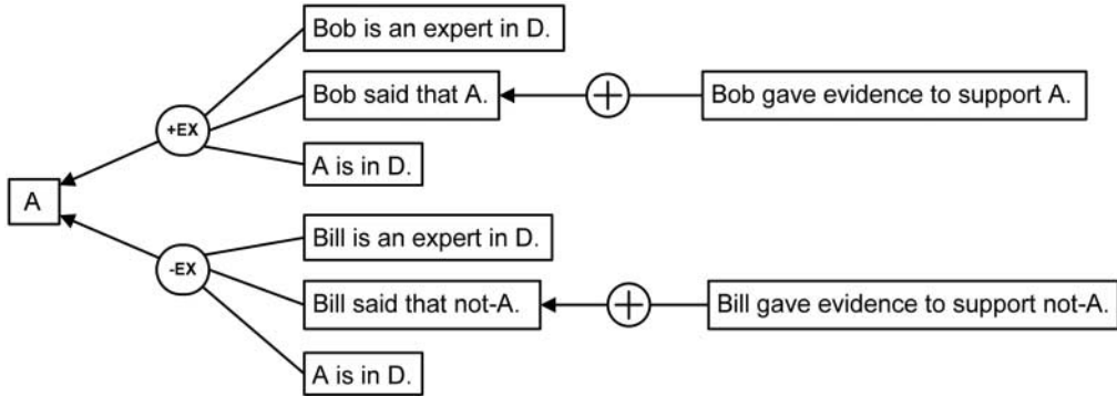
Figure 5. A case of the battle of the experts modelled in CAS.
