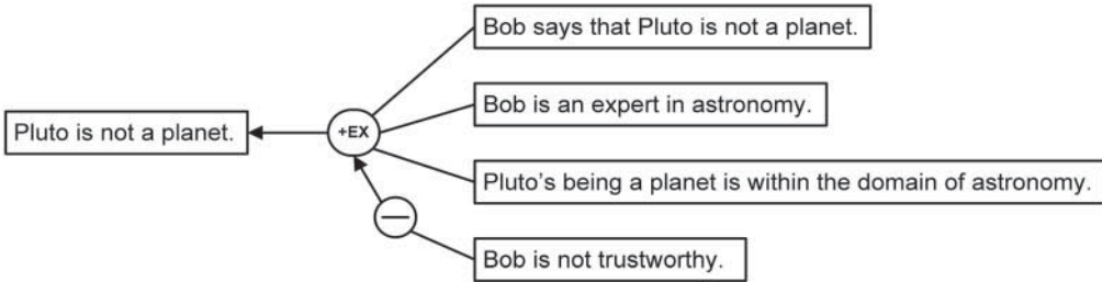
Figure 4. Carneades version of the Pluto example.
