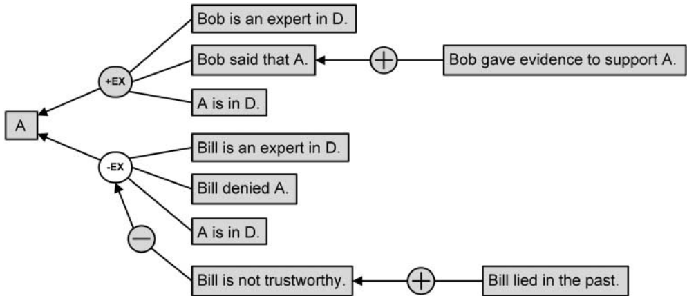
Figure 7. The trustworthiness critical question modelled as undercutter.
